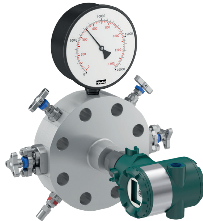
Monoflange with dual instrument (MFY170). Contact Parker.
